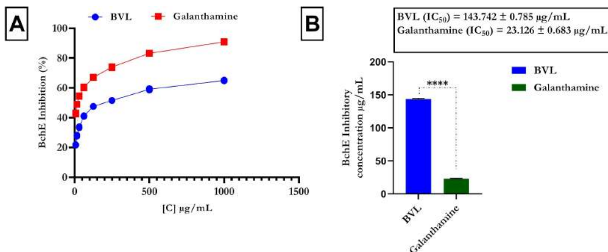
FIGURE 4 | Butyrylcholinesterase activity of B. vulgaris leaf flavonoid-rich extracts: (A) BchE percentage inhibitory activity and (B) inhibitory concentration ( \text{IC}_{50} ) values of BVL and galanthamine. Data are represented as the mean \pm SD ( n = 3 ); **** p < 0.0001 indicates an extremely significant difference compared with the standard drug (galanthamine). BVL, B. vulgaris leaf; galanthamine, standard drug.
