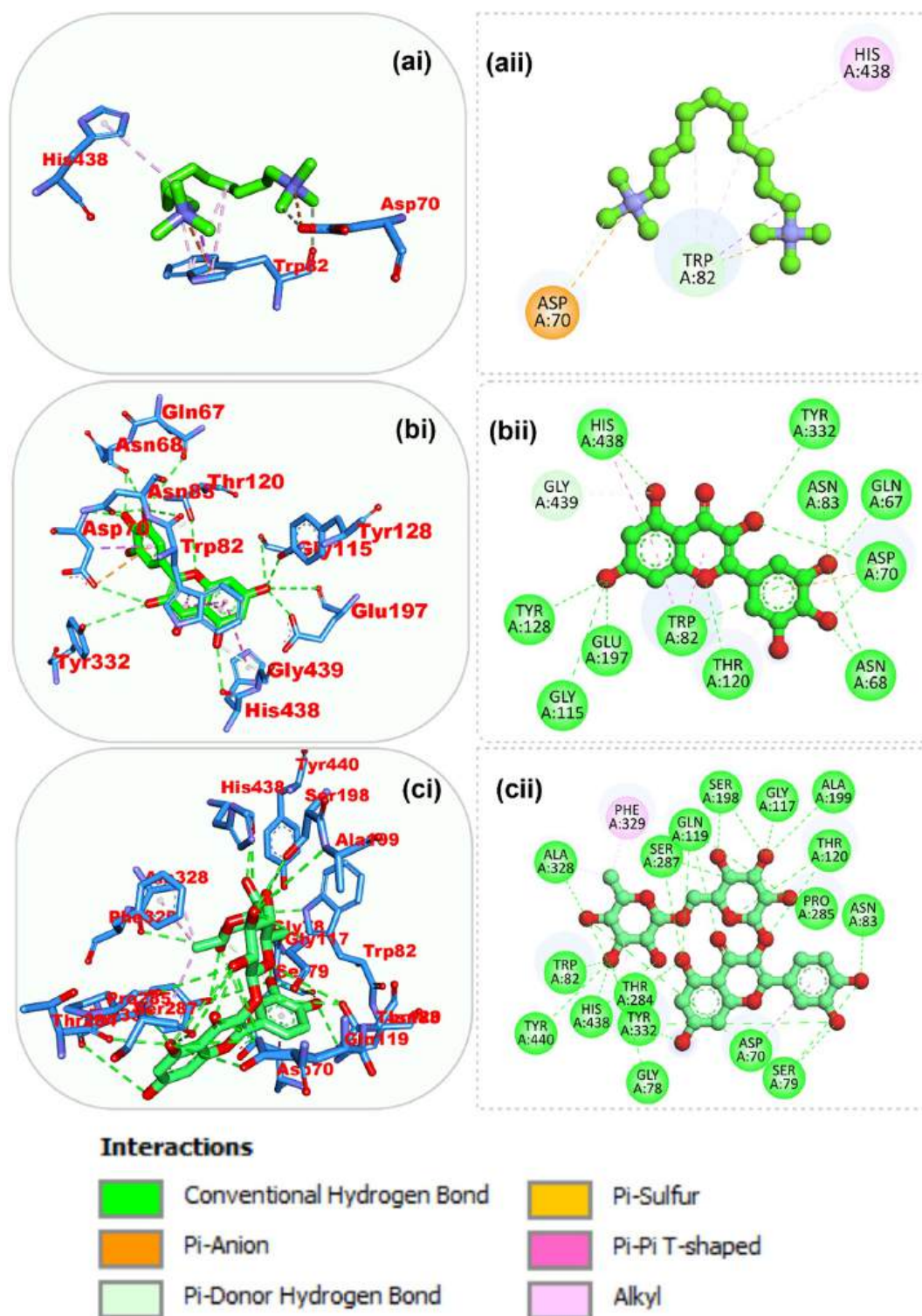
FIGURE 7 | Top scoring ligands (myricetin and rutin) and butylcholinestarse inhibitor (decamethonium) within the active site of protein 6EP4. This figure illustrates the binding interactions of the reference inhibitor decamethonium and the test ligands myricetin and rutin within the active site of human butylcholinesterase (BChE). Panels (a), (b), and (c) represent the ligands decamethonium, myricetin, and rutin, respectively, as shown in (i) The 3D binding pose shows its precise orientation and position within the enzyme's active site, highlighting key residues involved in hydrogen bonding, hydrophobic interactions, and other noncovalent forces. This view provides insight into the spatial complementarity between the ligand and the binding pocket. (ii) The 2D interaction representation details the specific amino acid residues of 6EP4 that form direct interactions with the ligand, along with the types of interactions (e.g., hydrogen bonds, pi-pi stacking, and van der Waals forces). This comprehensive visualization allows for a clear understanding of the molecular basis of ligand–enzyme recognition and provides crucial information for structure–activity relationship studies and future drug design efforts.
